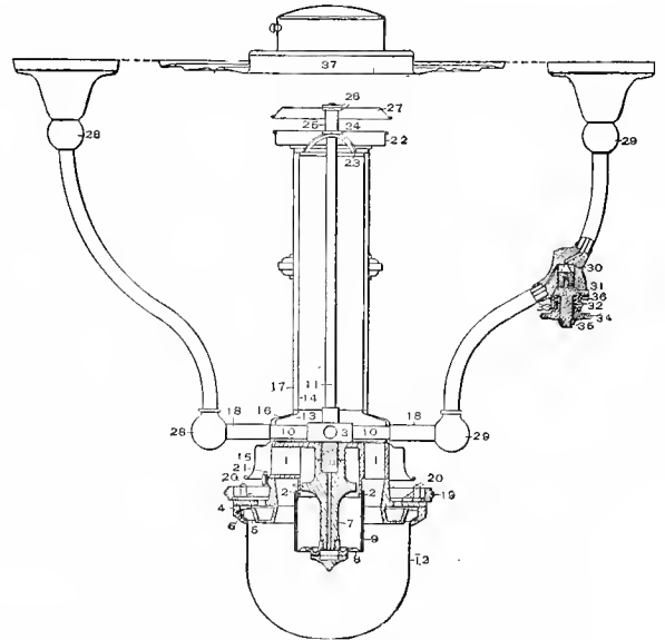
Fig. 3139. Section.
